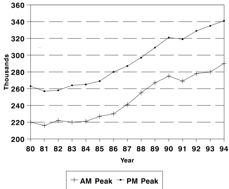
Figure 2. Total Travel in 000's Vehicle-kilometres ,7-9am & 4-6pm
