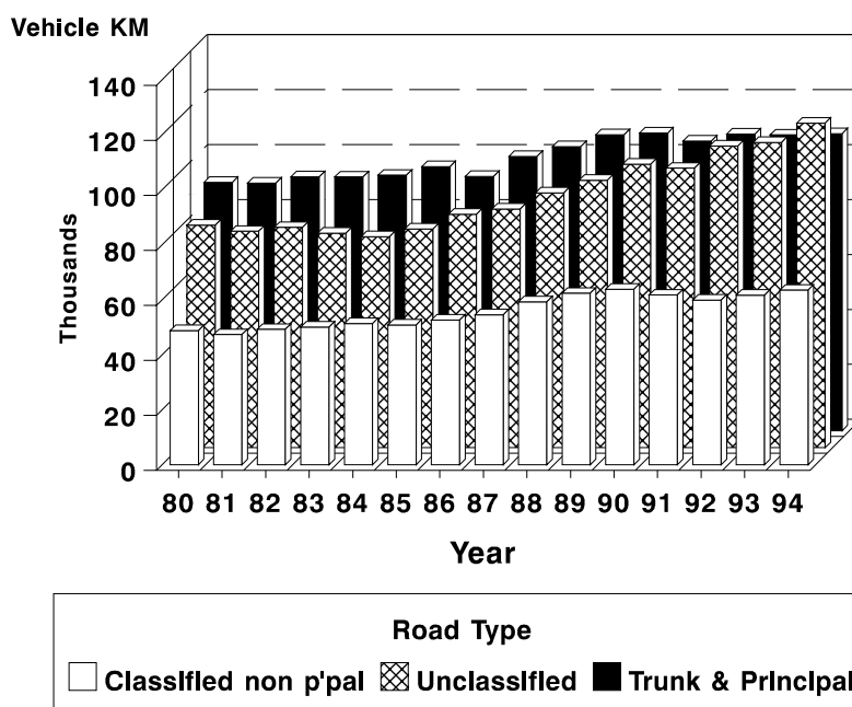
Figure 3 Total Travel in 000's Vehicle-kilometres, 7-9am Monday to Friday Average Day
