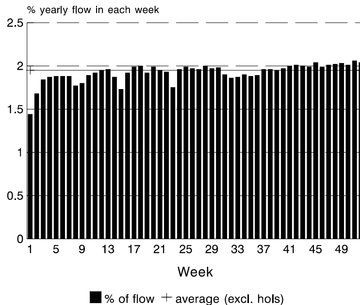
Figure 6. Seasonal Variations 1994. All Roads Except Motorways - 24 hour average day (Monday-Friday)
