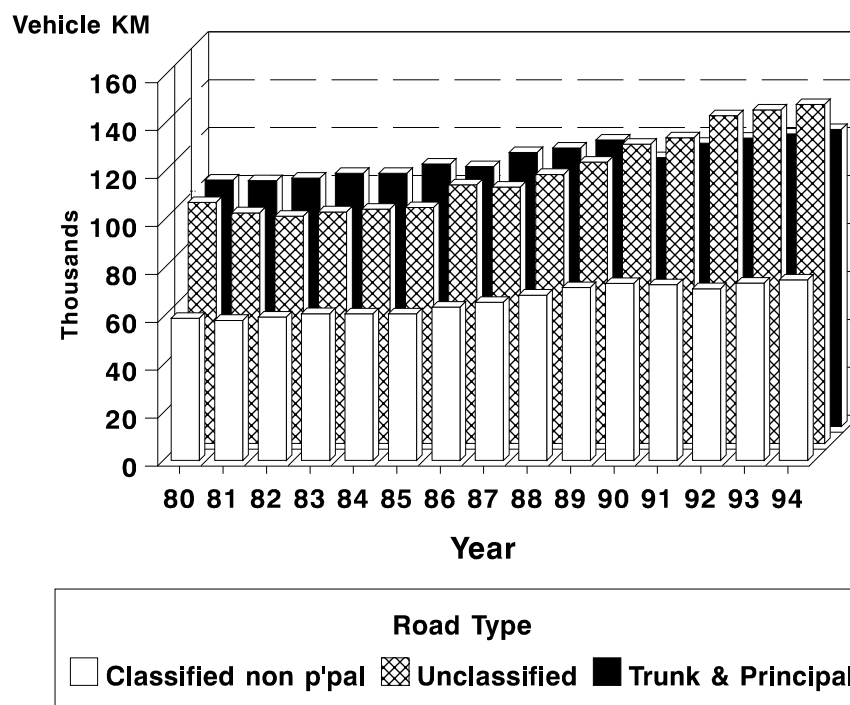
Figure 4 Total Travel in 000's Vehicle-kilometres, 4-6pm Monday to Friday Average Day
